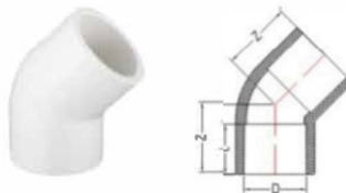
45 Degree Elbow
