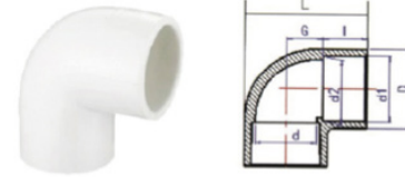
90 Degree Elbow
